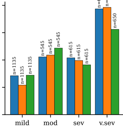
Moldova
